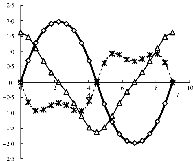
Figure 3. Comparison of results for the homogeneous Duffing equation of second order: \diamond , y GDQR; —, y equation (5); \triangle , y' GDQR; —, y' equation (5); \times , y'' GDQR; ---, y'' equation (5).
