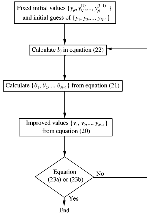
Figure 1. Diagram for the iterative solution procedure of second order Duffing equation.
