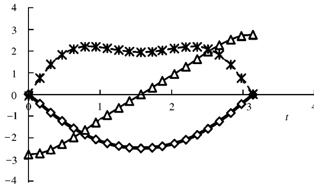
Figure 2. Comparison of results for the forced Duffing equation of second order: \diamond , y GDQR; —, y equation (3); \triangle , y' GDQR; —, y' equation (3); \times , y'' GDQR; ---, y'' equation (3).
